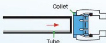
Diagram 3 - Tube Connections
