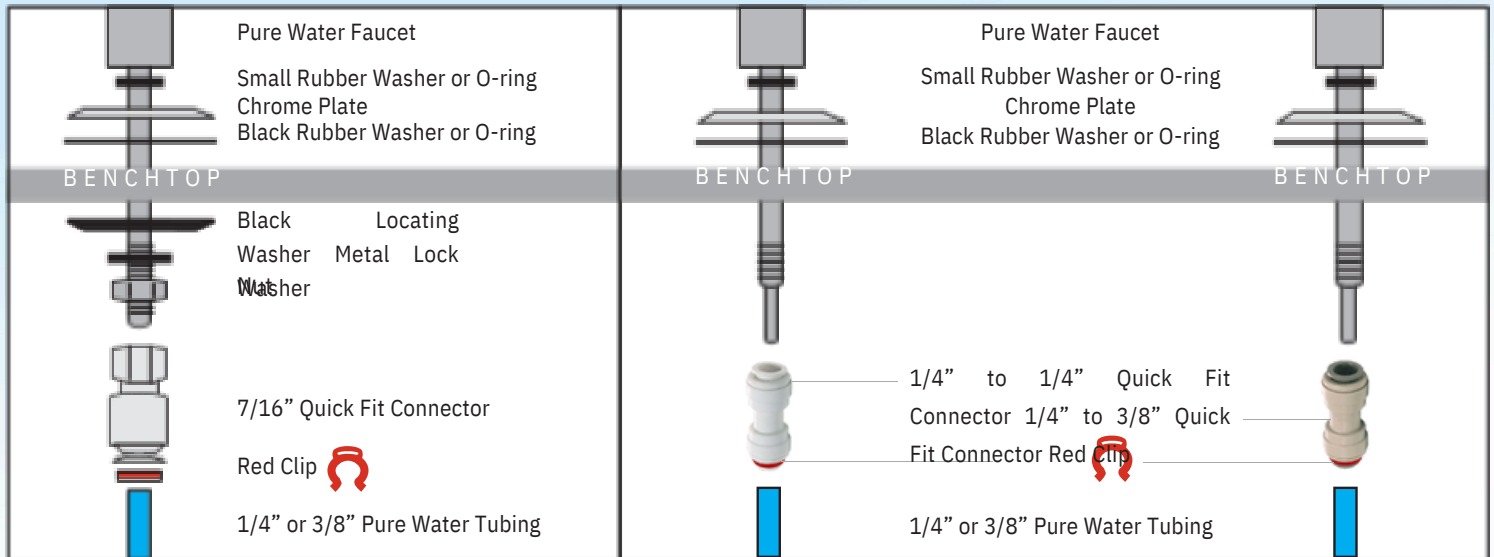
Diagram 4 - Faucet Installation
